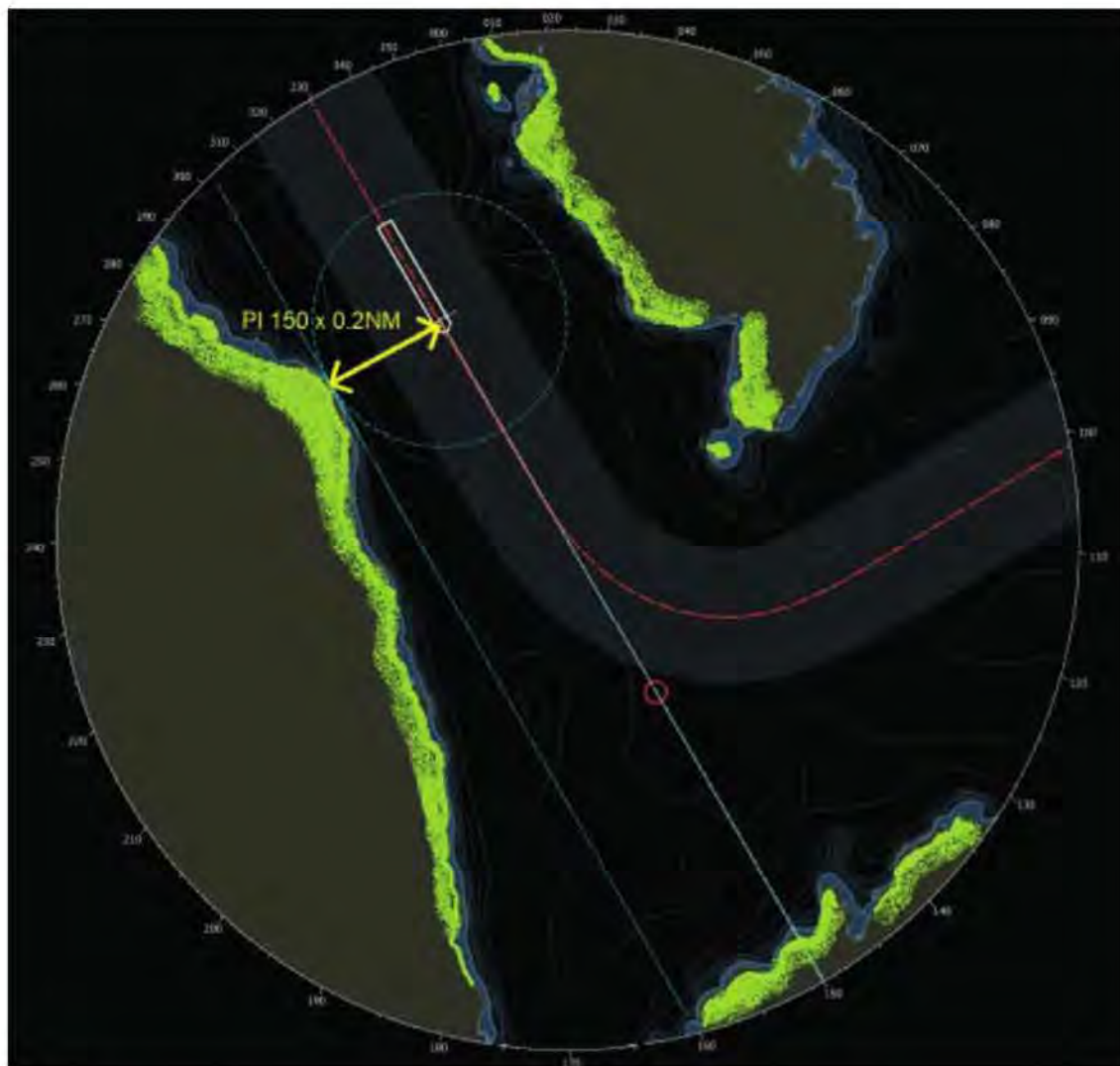
Figure 5.7: Parallel indexing radar on ECDIS
