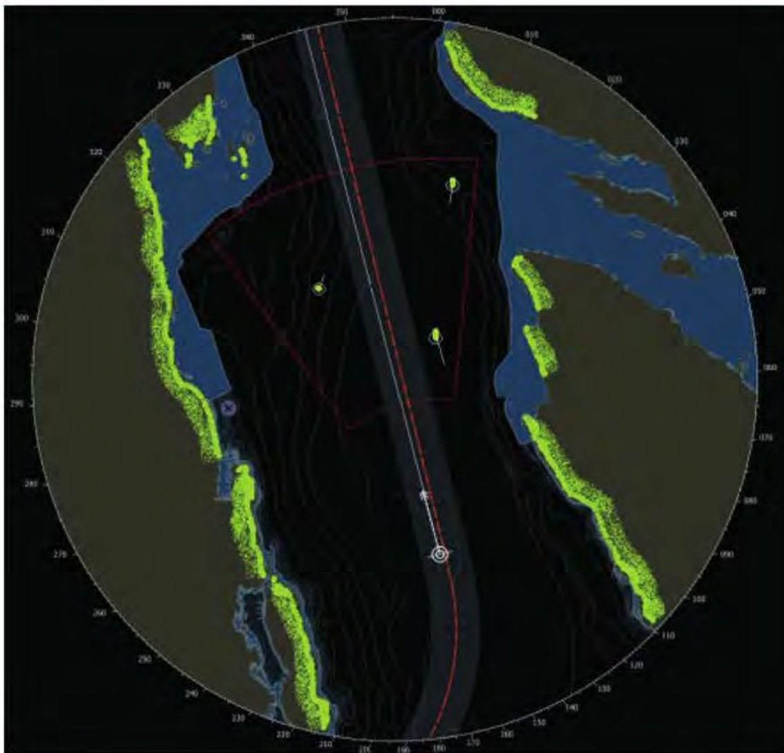
Figure 5.5: Automatic radar target acquisition on ECDIS
