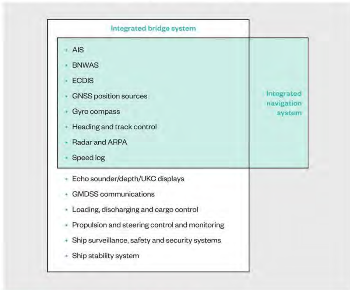
Figure 5.9: Systems integrated into an IBS and INS
