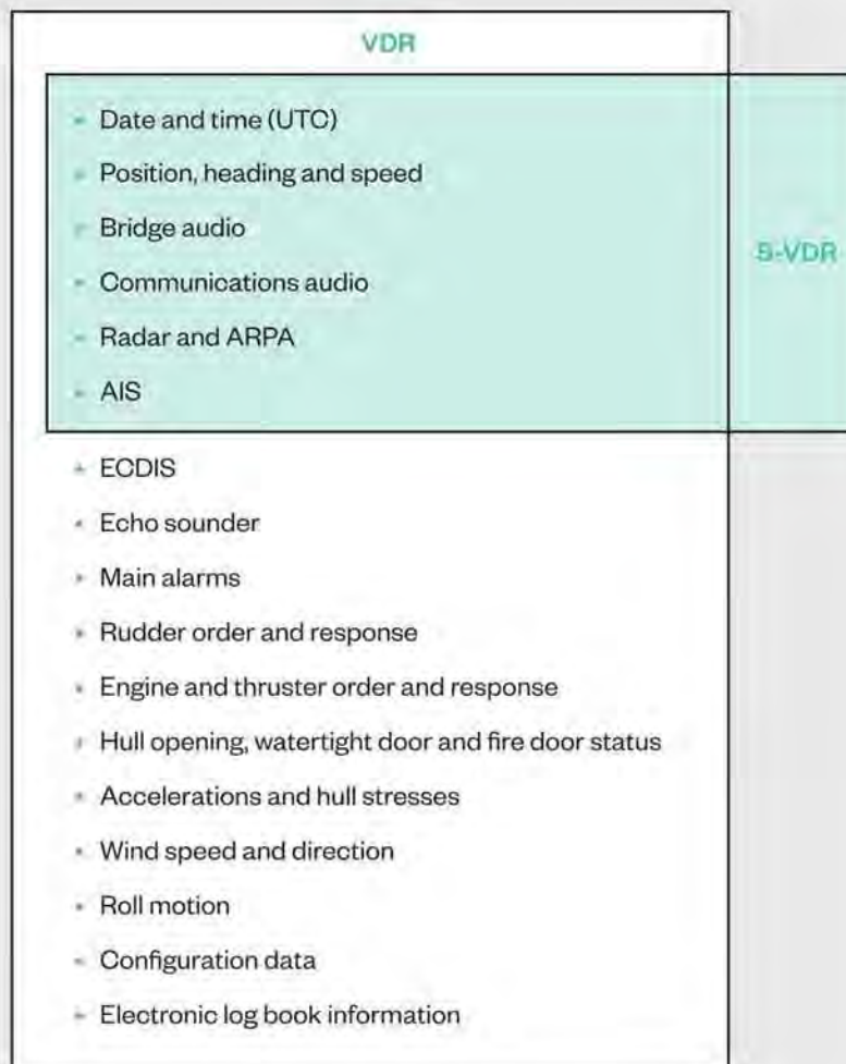
Figure 5.2: Data recorded in a VDR
