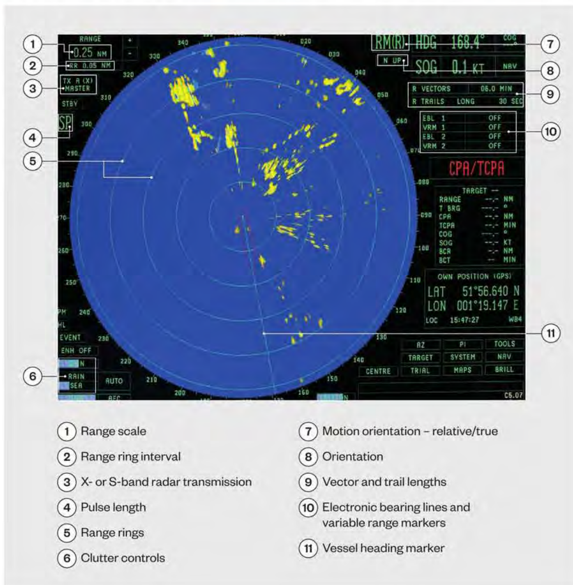
Figure 5.4: Container ship radar screen
