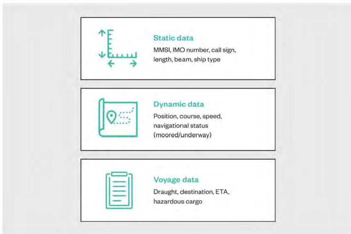
Figure 5.3: AIS information transmitted by a VHF broadcast system
