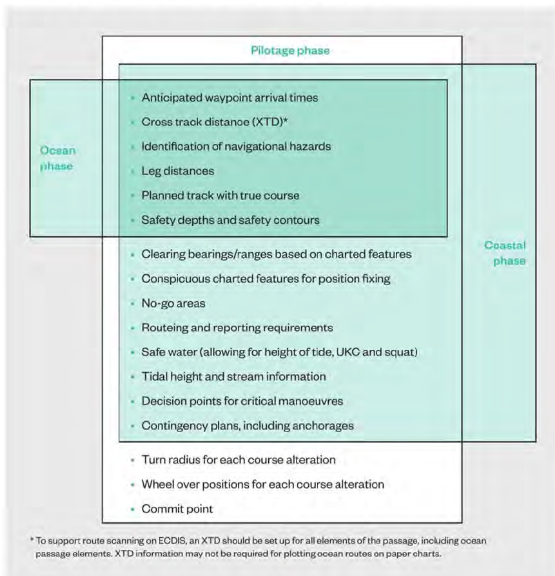
Figure 3.5: Information to show in route plotting
