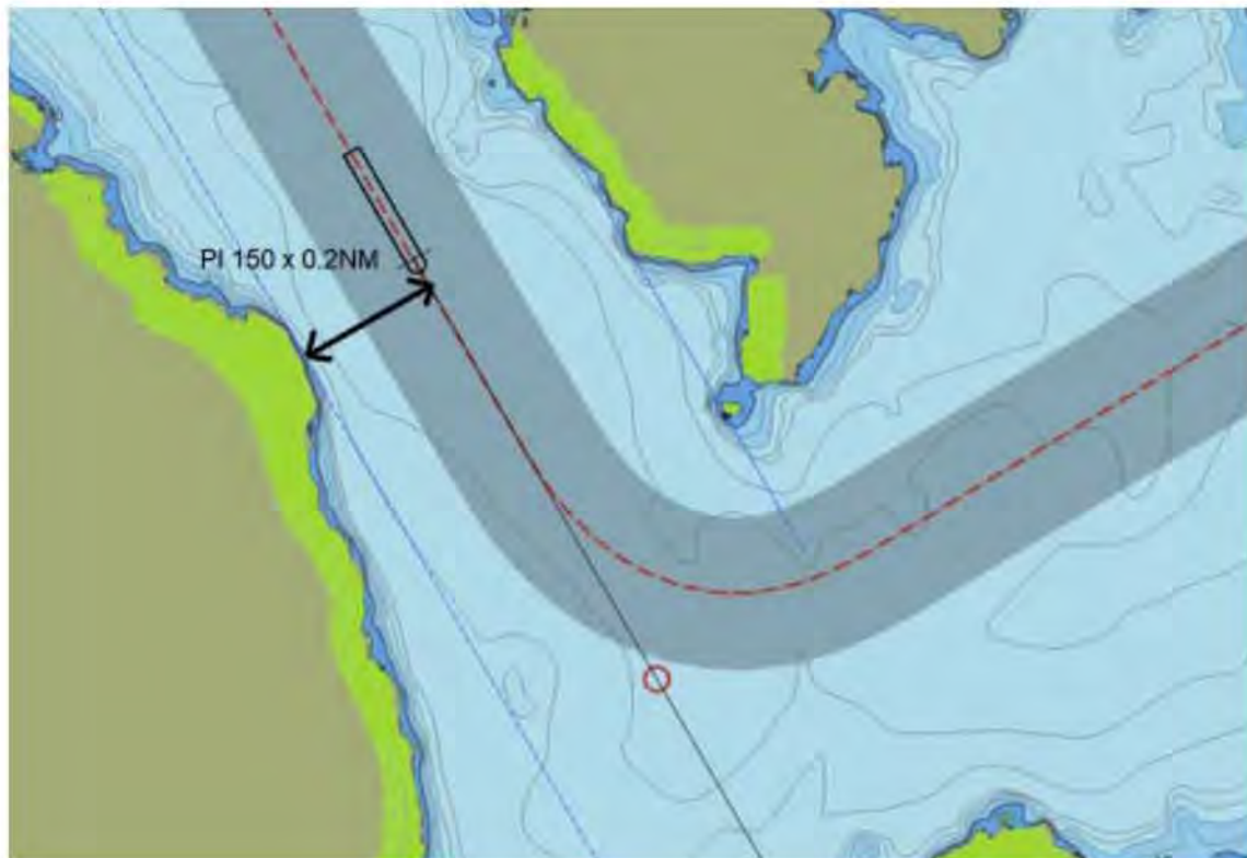
Figure 5.6: Parallel indexing on ECDIS
