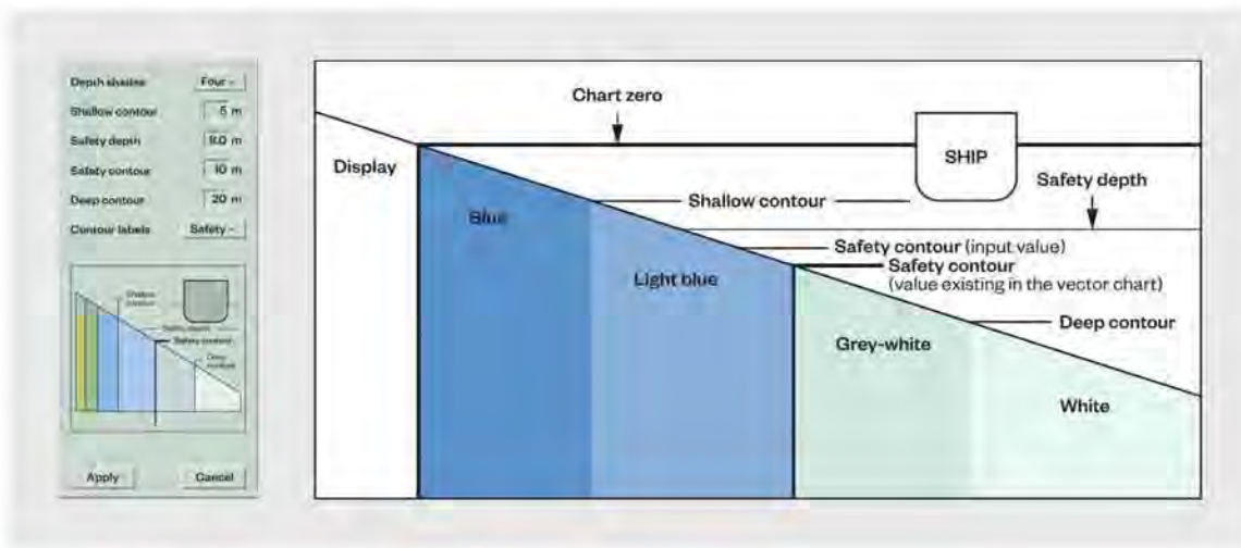
Figure 3.6: How contour lines indicate navigable waters
