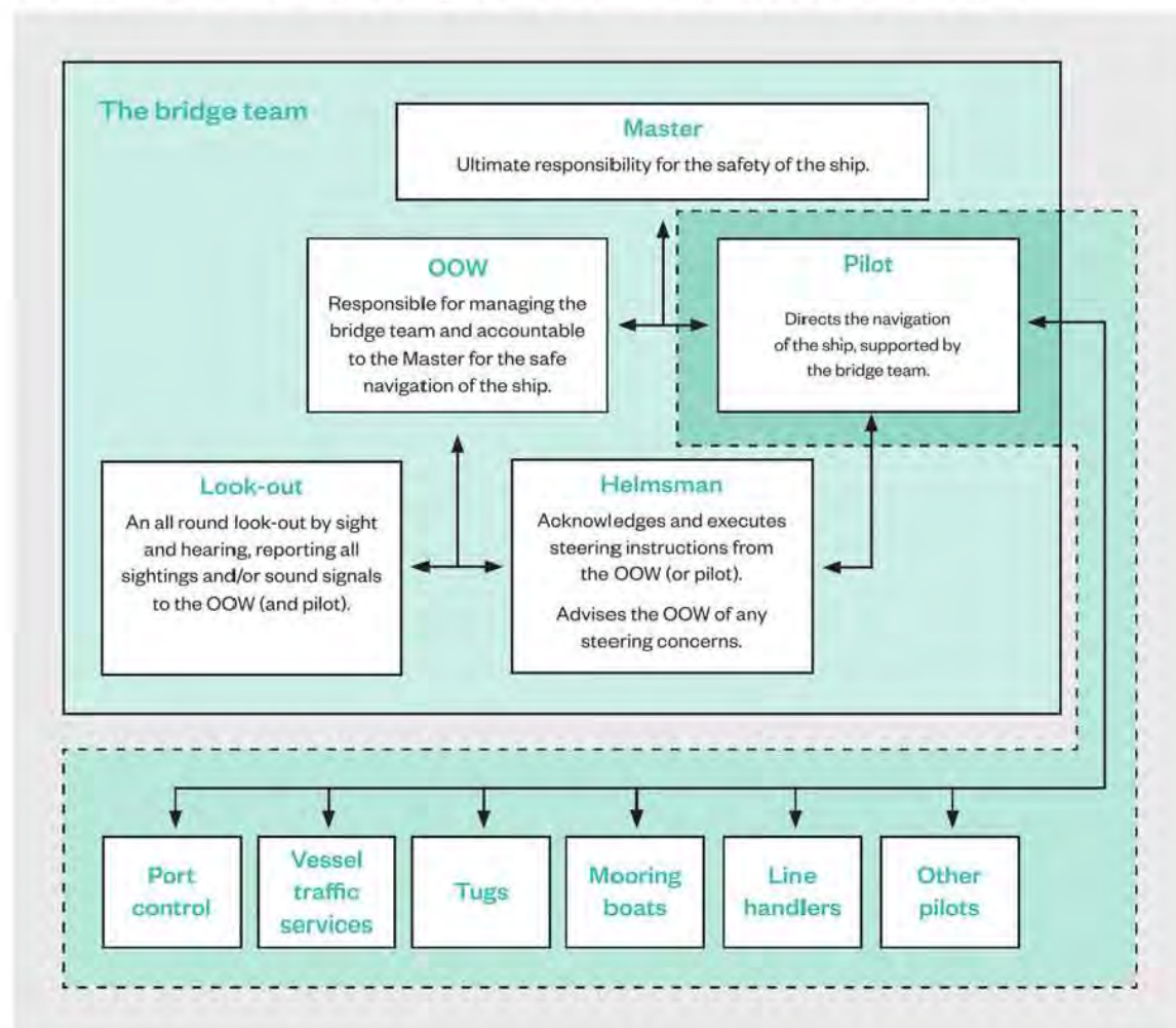
Figure 6.2: Example of bridge team/pilot co-operation
